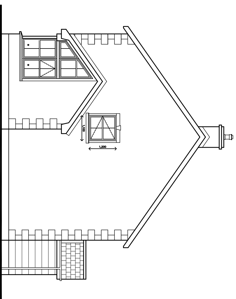
....side elevation
